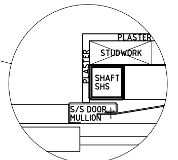
STANDARD DOOR SETOUT (CAN VARY)
